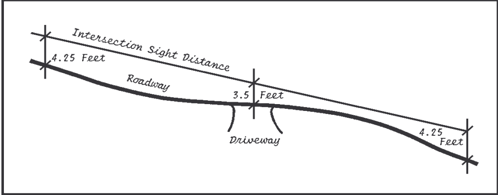
Figure 22-3: Measurement of Vertical Intersection Sight Distance
