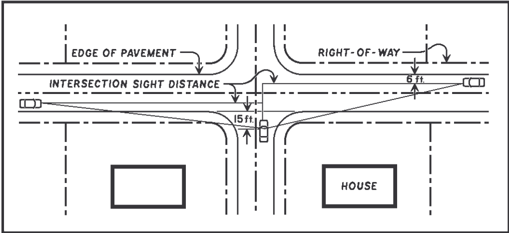
Figure 22-2: Measurement of Horizontal Intersection Sight Distance
