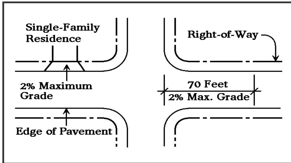
Figure 22-1: Diagram Illustrating Measurement of Grade at an Intersection
